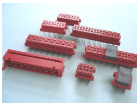
DS3900 series Mini connector red, pitch 1.27 mm. (flatcable-to-board connector series)
